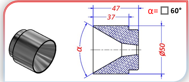
Pressure RS 25 die in steel DK 25
