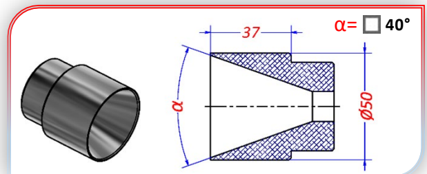
Tube RS 25 die in steel DT 25
