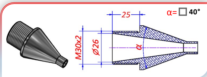
Tube RS 25 tip in steel TT 25
