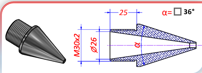
Semi-pressure RS 25 tip in steel TS 25
