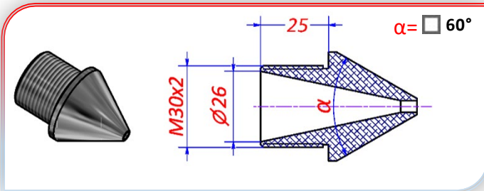
Pressure RS 25 tip in steel TK 25
